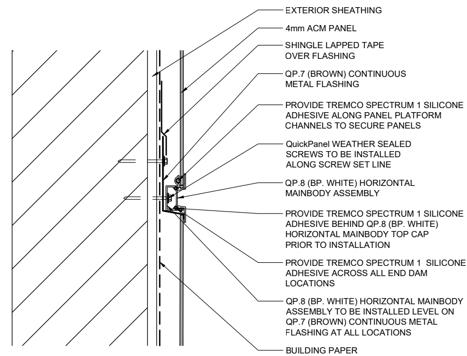
4 QuickPanel TYPICAL HORIZONTAL SECTION SCALE: 3" = 1'-0"
