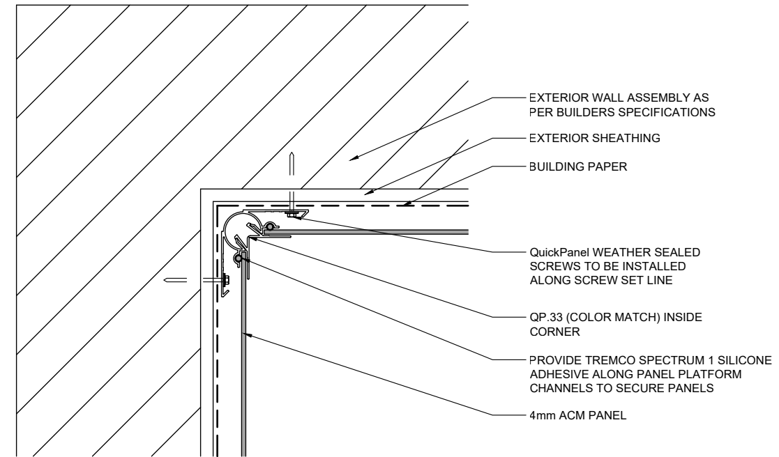
3 QuickPanel TYPICAL INSIDE CORNER SCALE: 3" = 1'-0"
