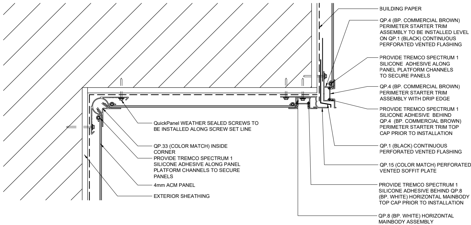
9A QuickPanel TYPICAL SOFFIT SECTION
