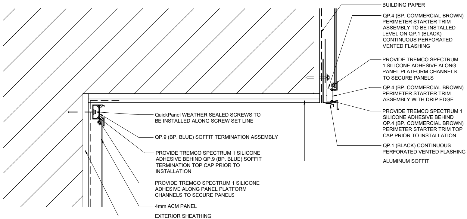
9B QuickPanel ALTERNATE SOFFIT SECTION
