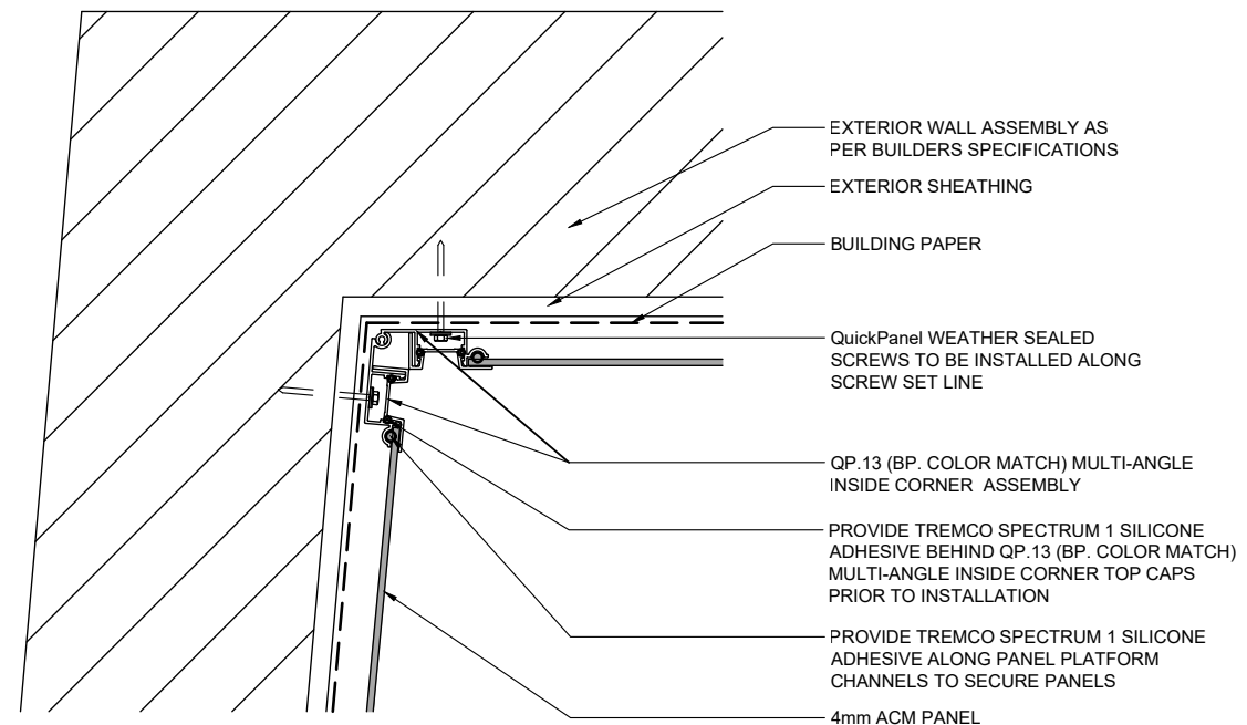
5 QuickPanel TYPICAL MULTI-ANGLE INSIDE CORNER SCALE: 3" = 1'-0"
