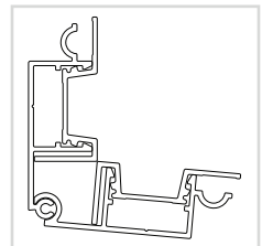
QP.13 Multi-Angle Inside Corner Assembly
