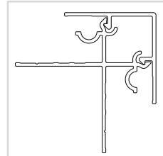
QP.2 Arrow Outside Corner Assembly
