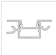
QP.11 Vertical Window Side Assembly
