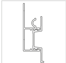
QP.4 Perimeter Starter Trim Assembly
